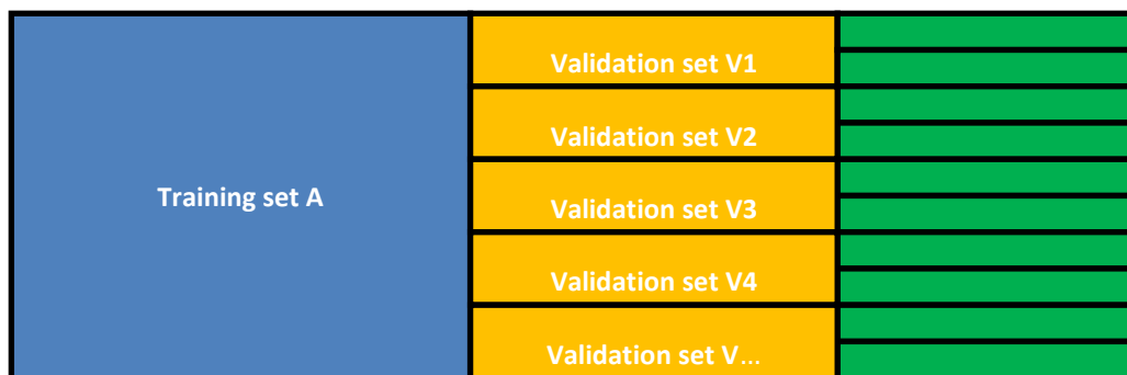
Figure 4.1. Training, Validation and Test Sets
