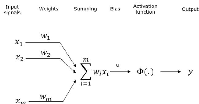
Figure 2.4. Artificial Neuron
